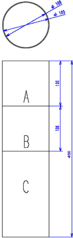
Figure 3: Dimensions of the landmarks (beacons)
