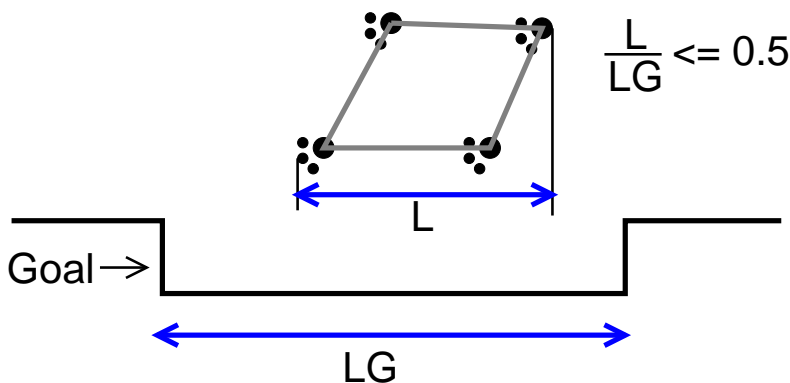
Figure 13: Illegal Defence
