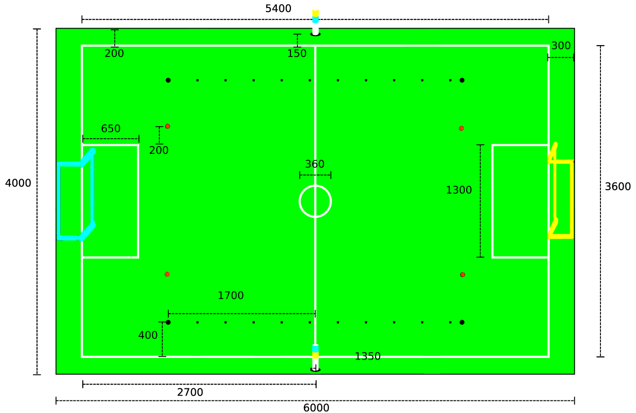
Figure 1: Scale diagram of entire field (dimensions in mm).
