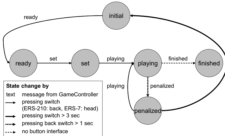
Figure 9: Robot states.
