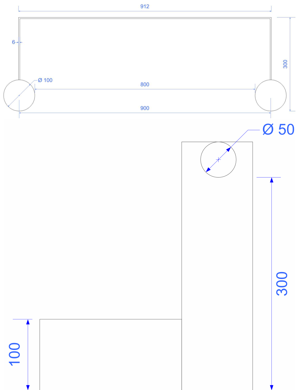
Figure 2: Dimensions of the new goal (without crossbar), viewed from above and from the side
